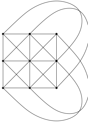
Figure 1.3: AG(2, 3)
